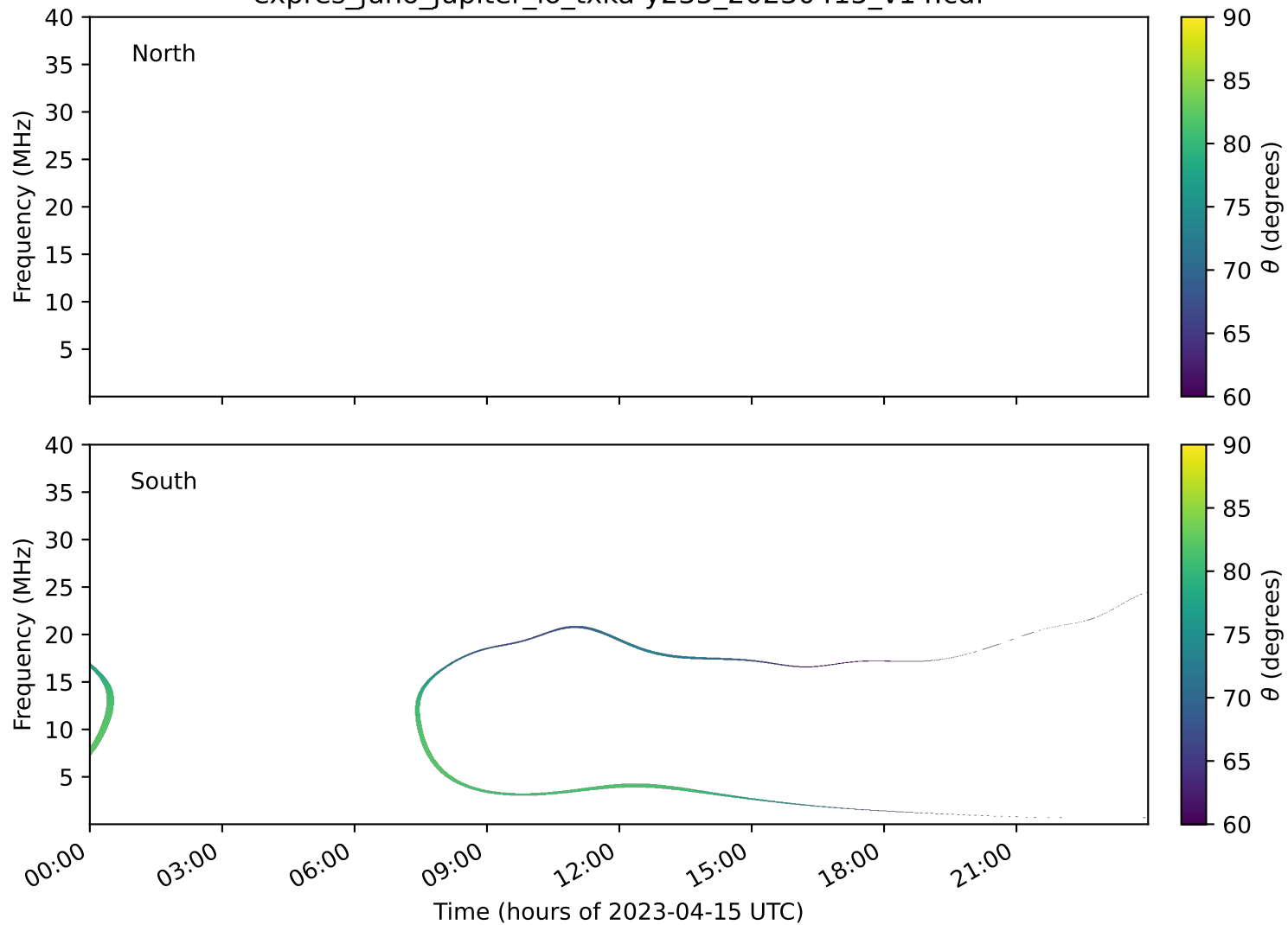
expres_juno_jupiter_io_txka-y235_20230415_v14.cdf
