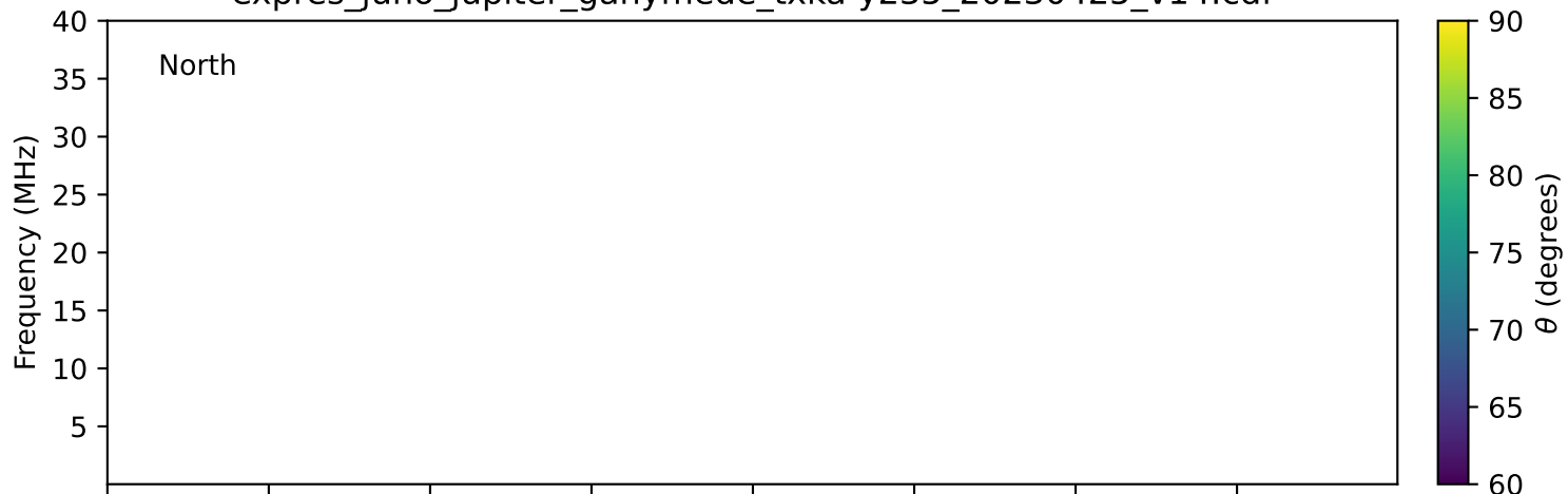
expres_juno_jupiter_ganymede_txka-y235_20230425_v14.cdf
