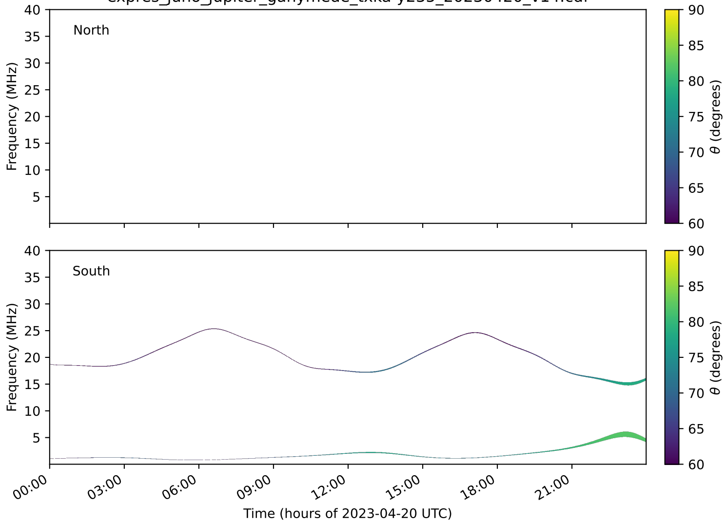
expres_juno_jupiter_ganymede_txka-y235_20230420_v14.cdf
