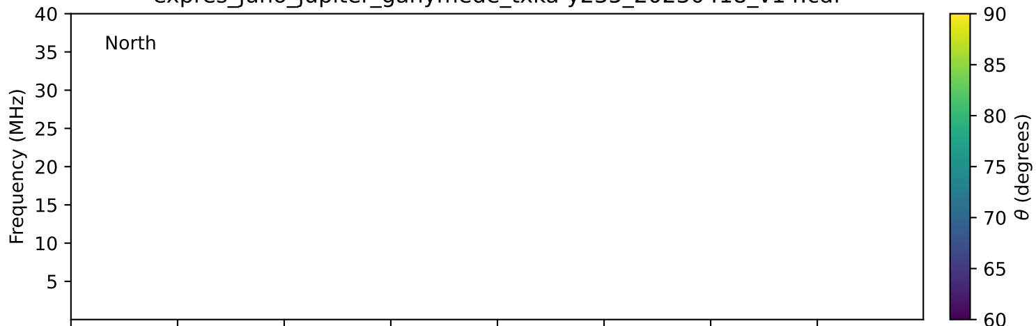
expres_juno_jupiter_ganymede_txka-y235_20230418_v14.cdf
