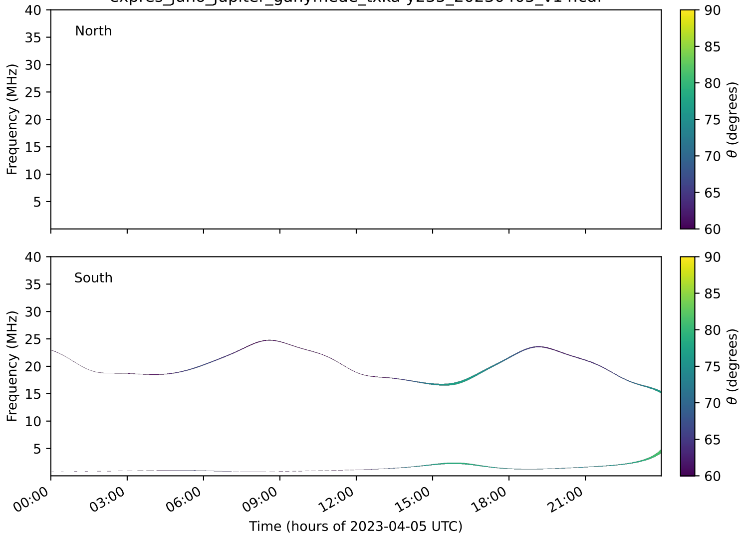
expres_juno_jupiter_ganymede_txka-y235_20230405_v14.cdf
