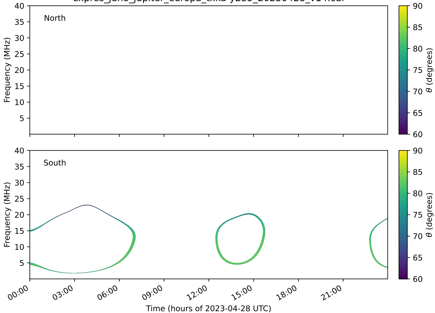
expres_juno_jupiter_europa_txka-y235_20230428_v14.cdf
