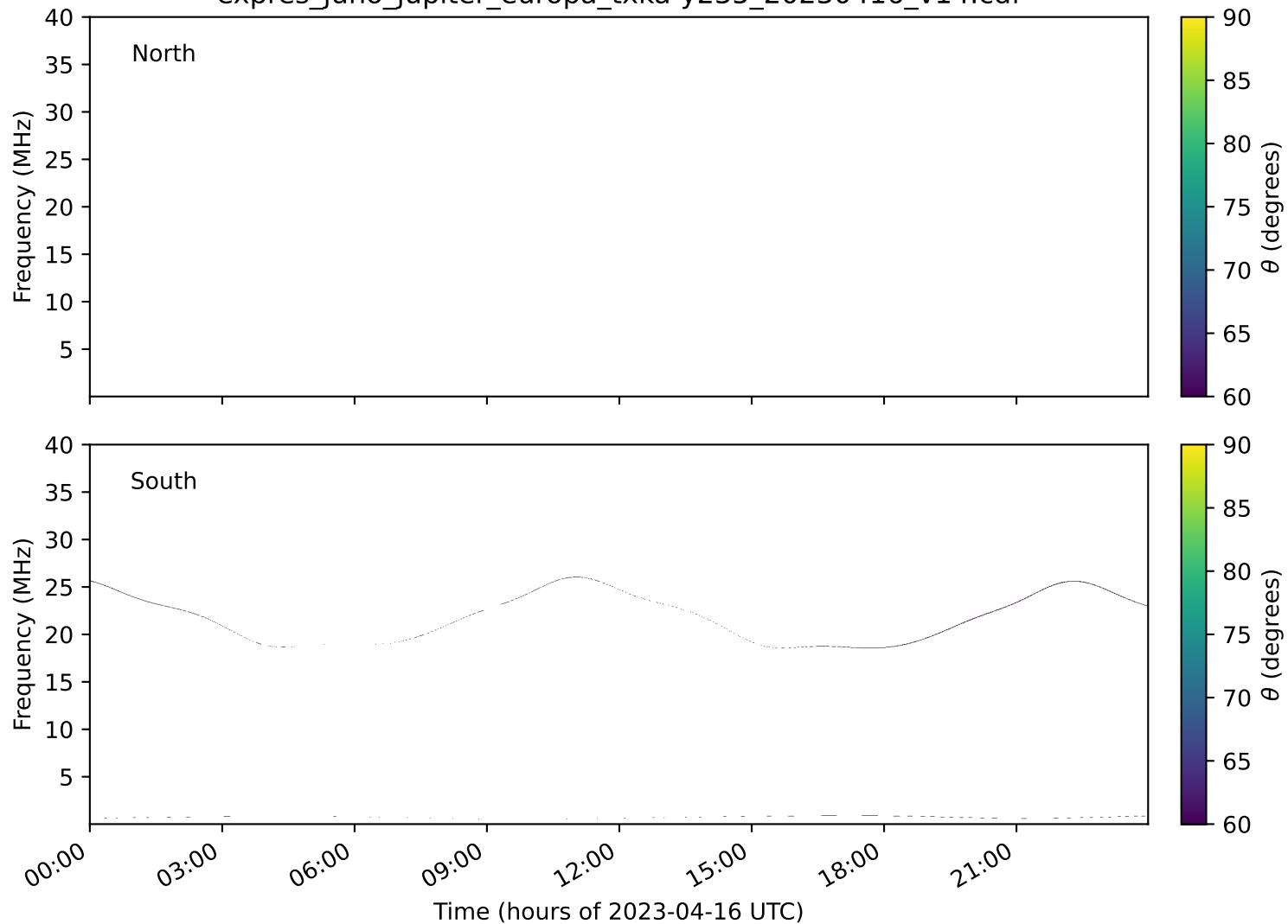
expres_juno_jupiter_europa_txka-y235_20230416_v14.cdf
