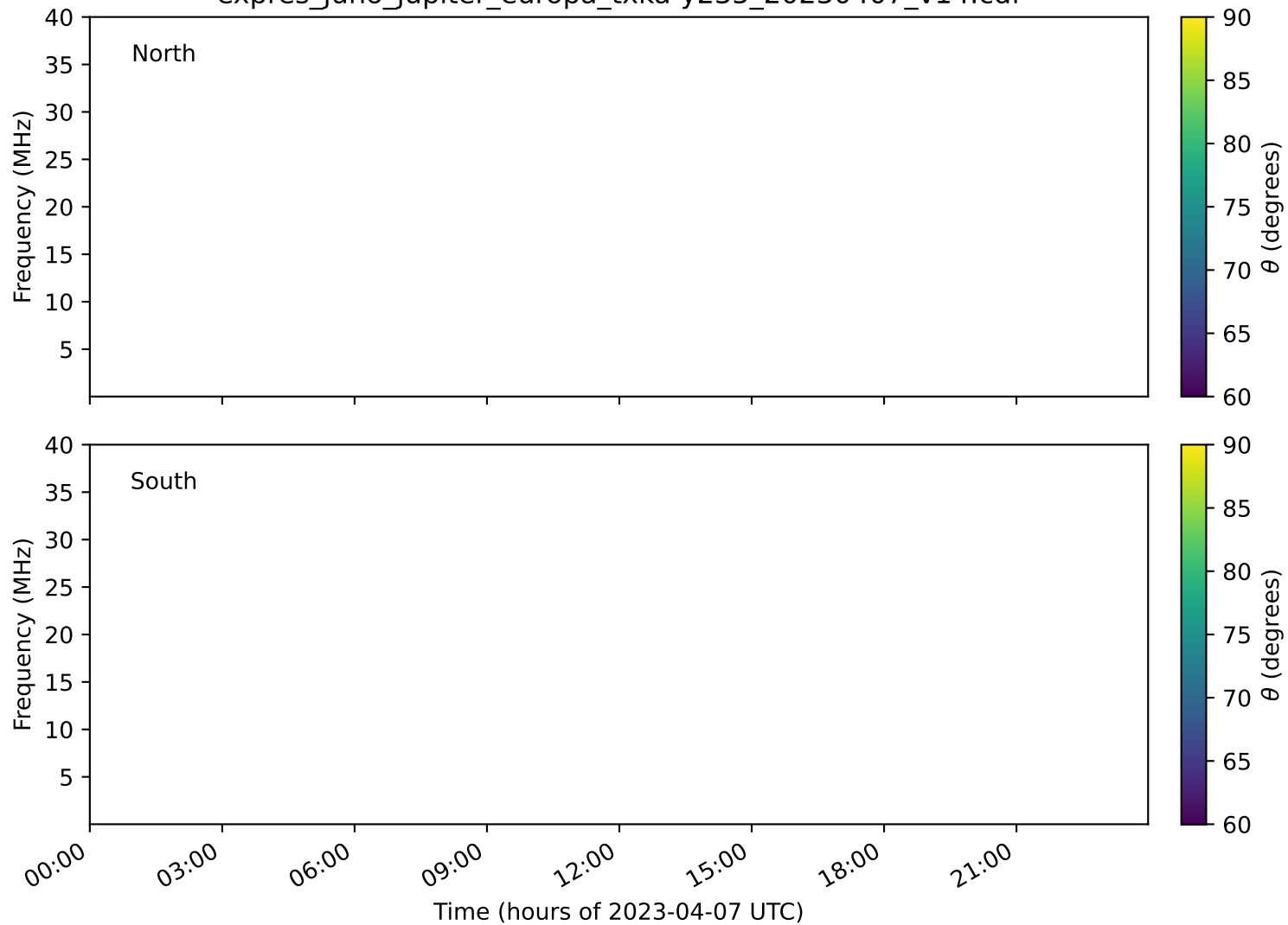
expres_juno_jupiter_europa_txka-y235_20230407_v14.cdf
