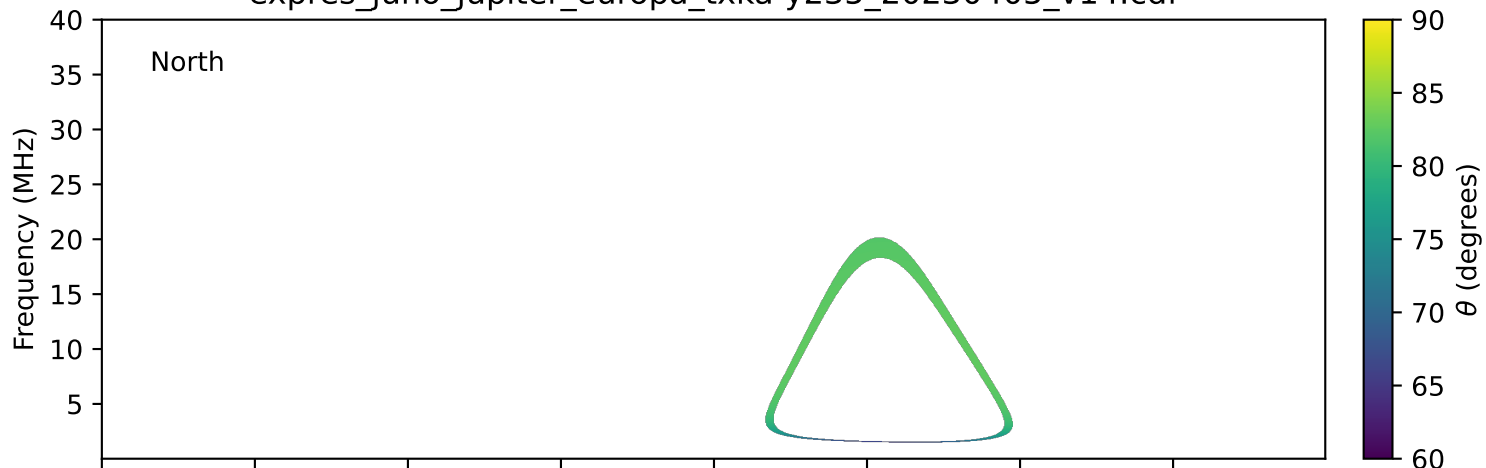
expres_juno_jupiter_europa_txka-y235_20230405_v14.cdf
