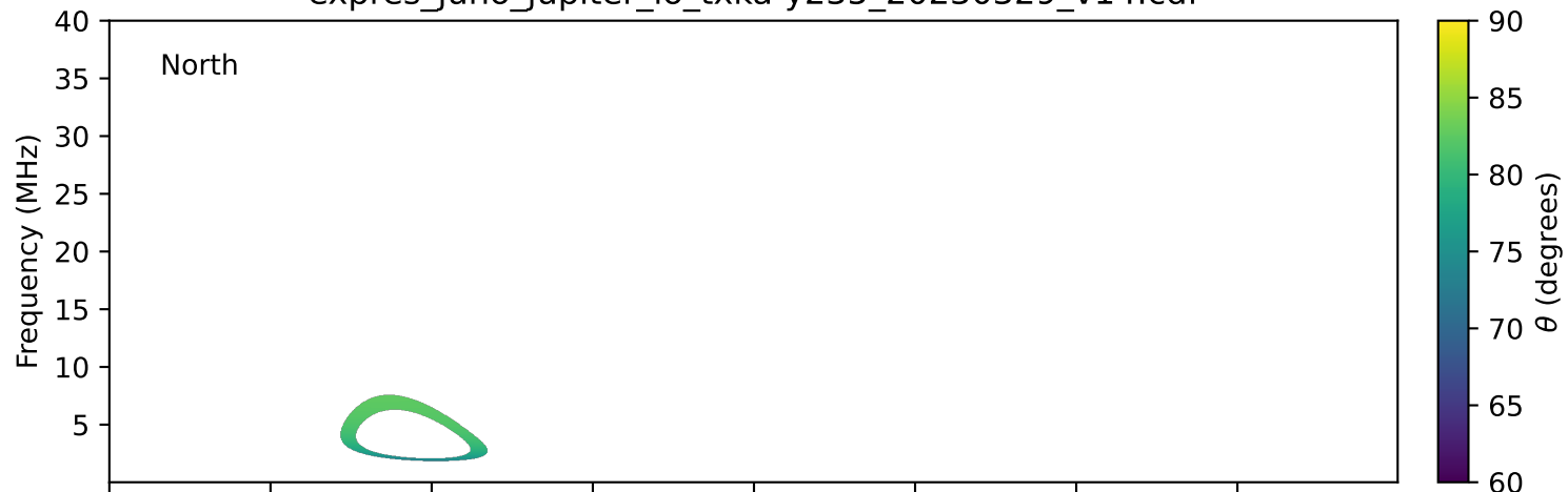
expres_juno_jupiter_io_txka-y235_20230329_v14.cdf
