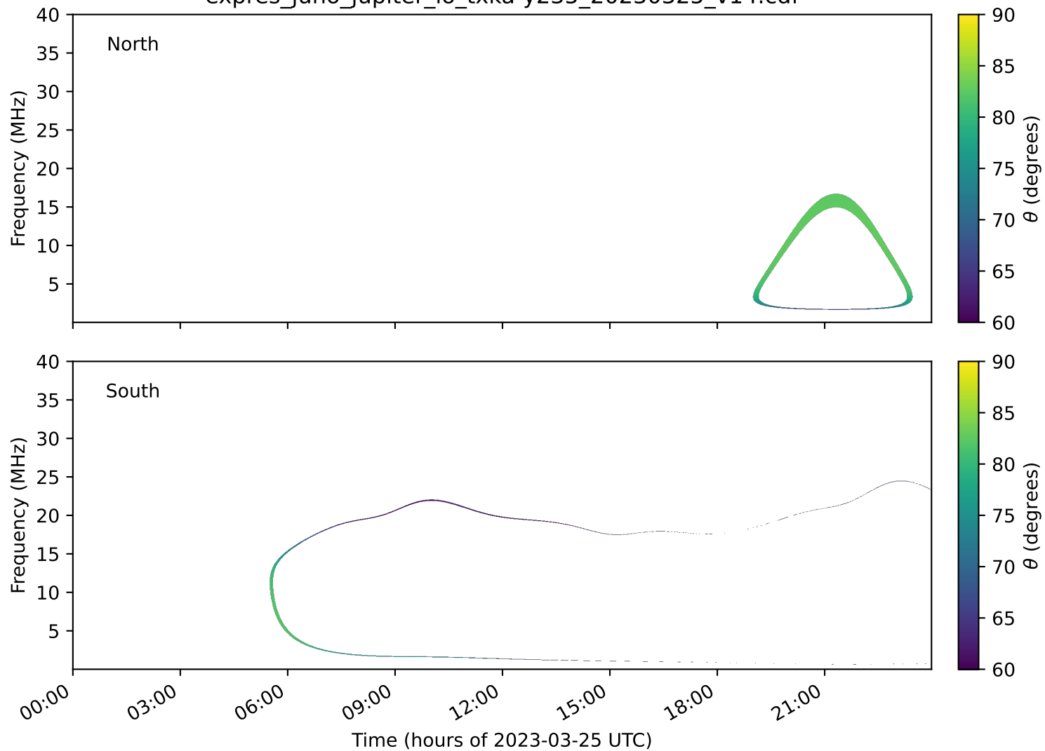
expres_juno_jupiter_io_txka-y235_20230325_v14.cdf
