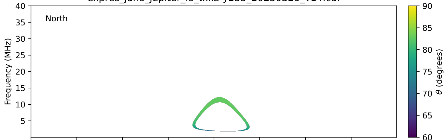
expres_juno_jupiter_io_txka-y235_20230320_v14.cdf
