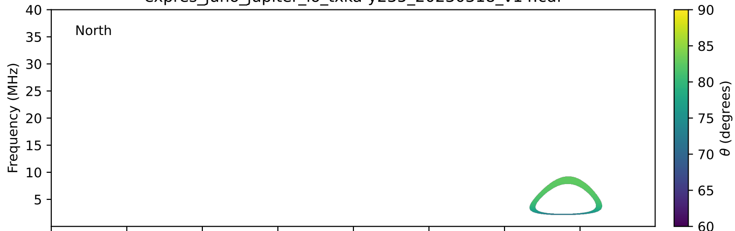
expres_juno_jupiter_io_txka-y235_20230318_v14.cdf
