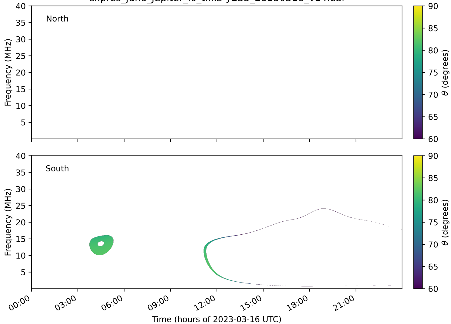
expres_juno_jupiter_io_txka-y235_20230316_v14.cdf
