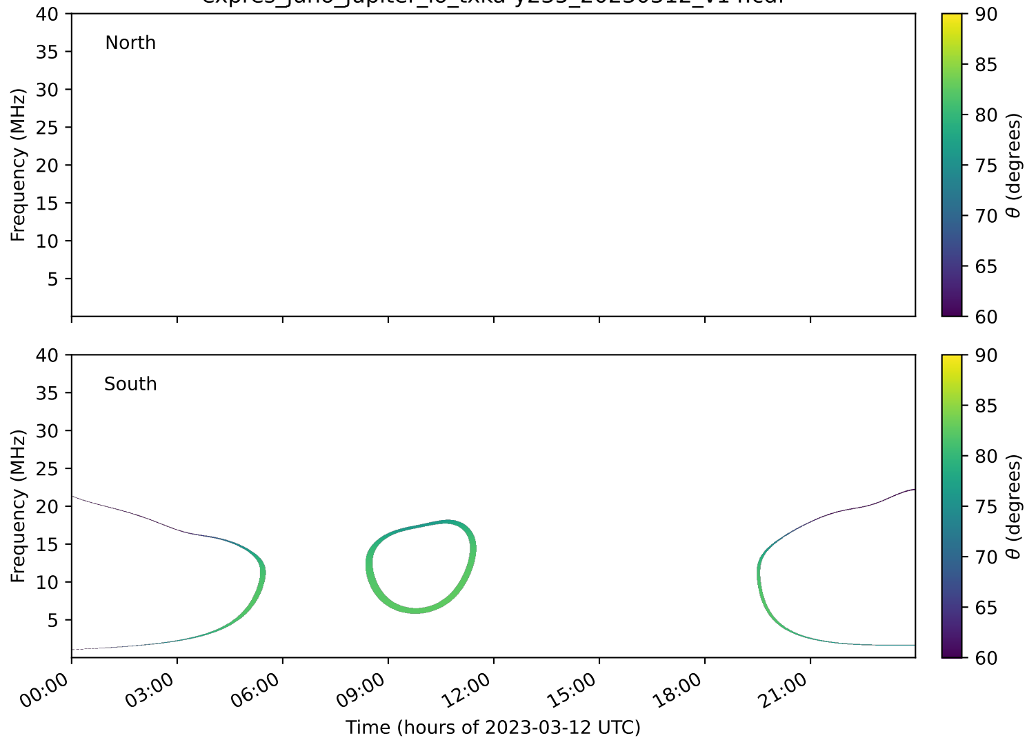
expres_juno_jupiter_io_txka-y235_20230312_v14.cdf
