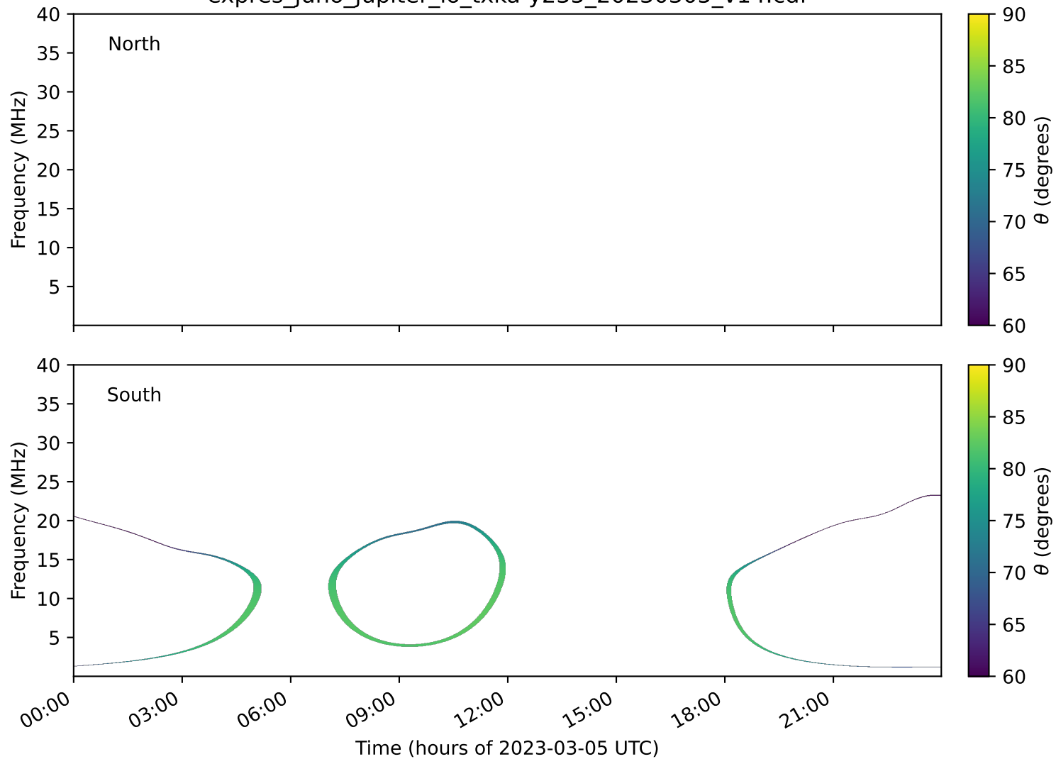
expres_juno_jupiter_io_txka-y235_20230305_v14.cdf
