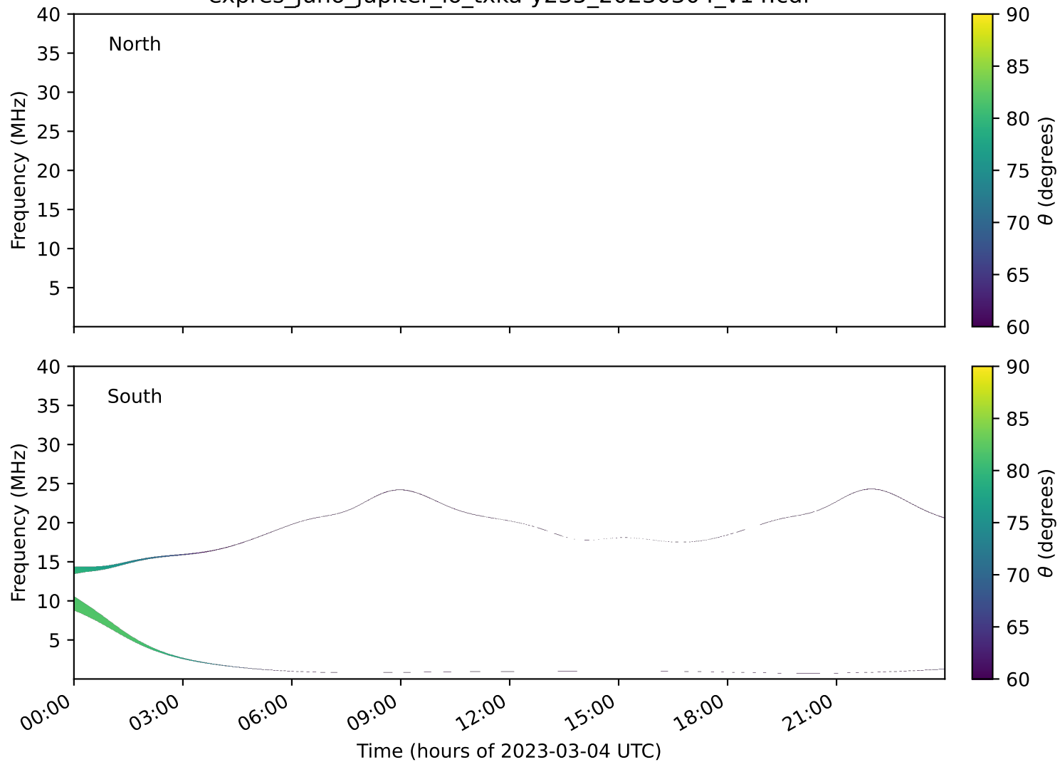
expres_juno_jupiter_io_txka-y235_20230304_v14.cdf
