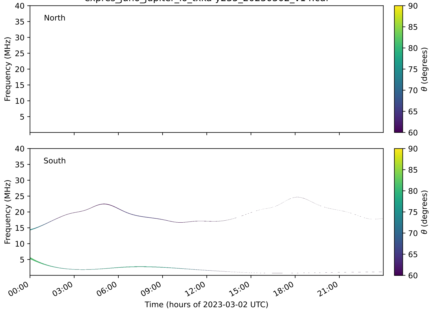
expres_juno_jupiter_io_txka-y235_20230302_v14.cdf
