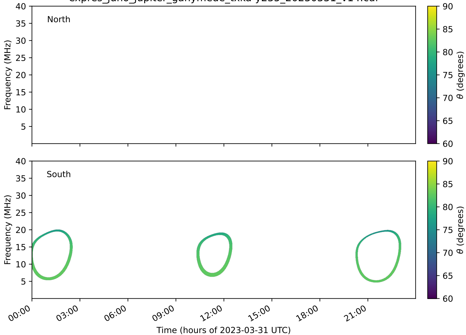
expres_juno_jupiter_ganymede_txka-y235_20230331_v14.cdf
