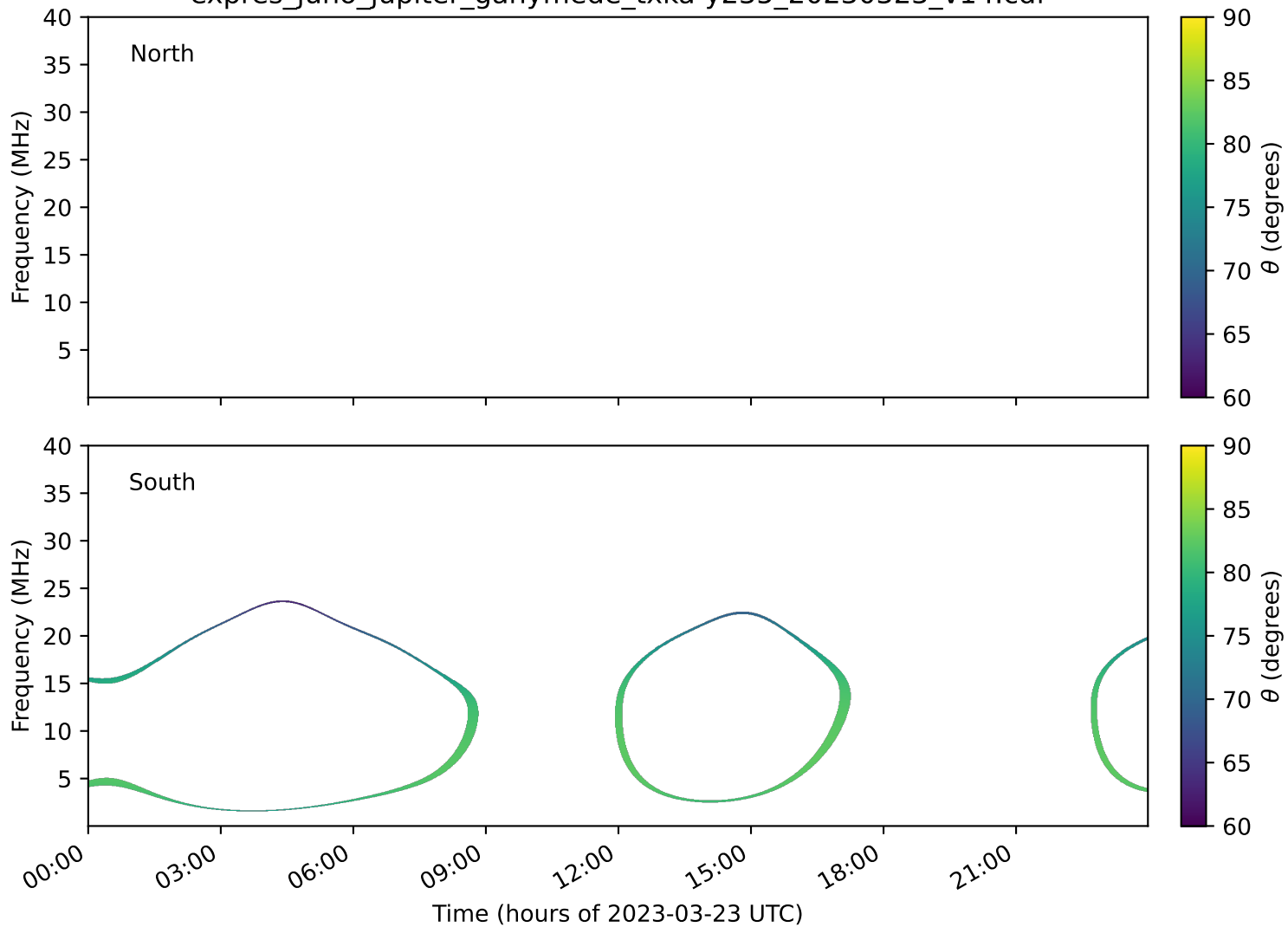
expres_juno_jupiter_ganymede_txka-y235_20230323_v14.cdf
