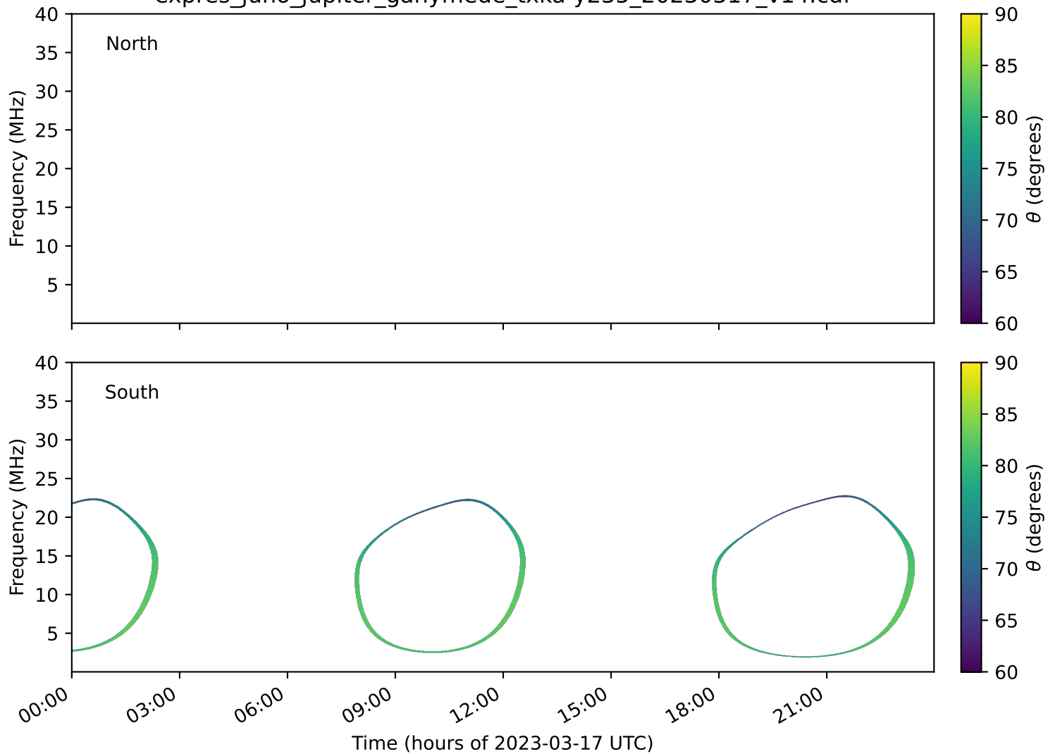
expres_juno_jupiter_ganymede_txka-y235_20230317_v14.cdf
