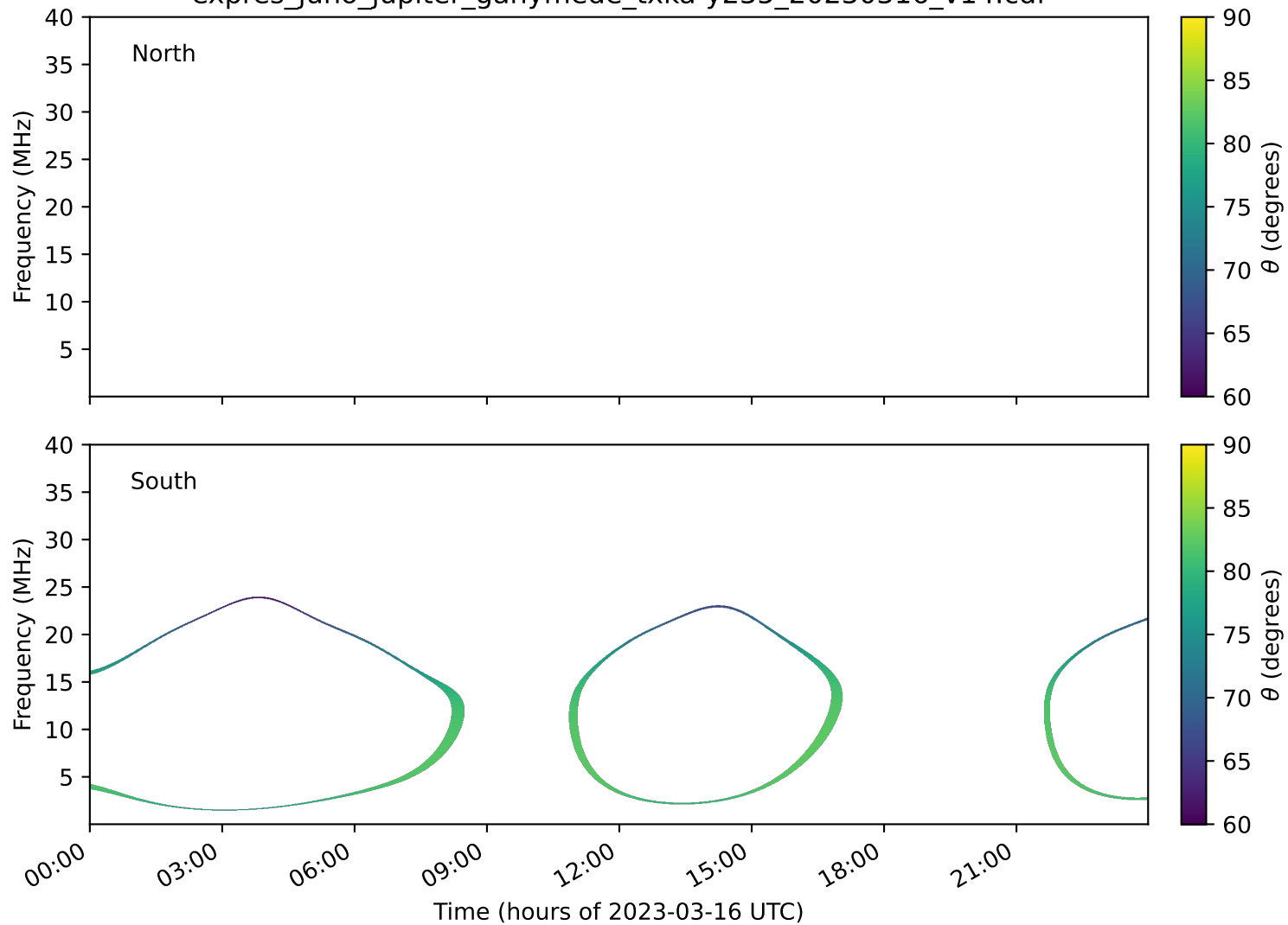
expres_juno_jupiter_ganymede_txka-y235_20230316_v14.cdf
