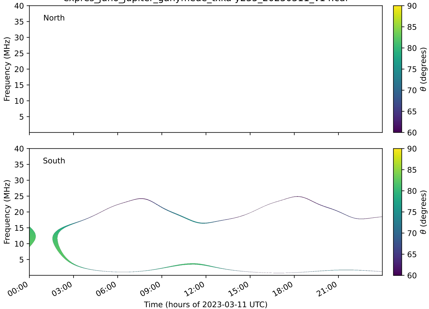
expres_juno_jupiter_ganymede_txka-y235_20230311_v14.cdf
