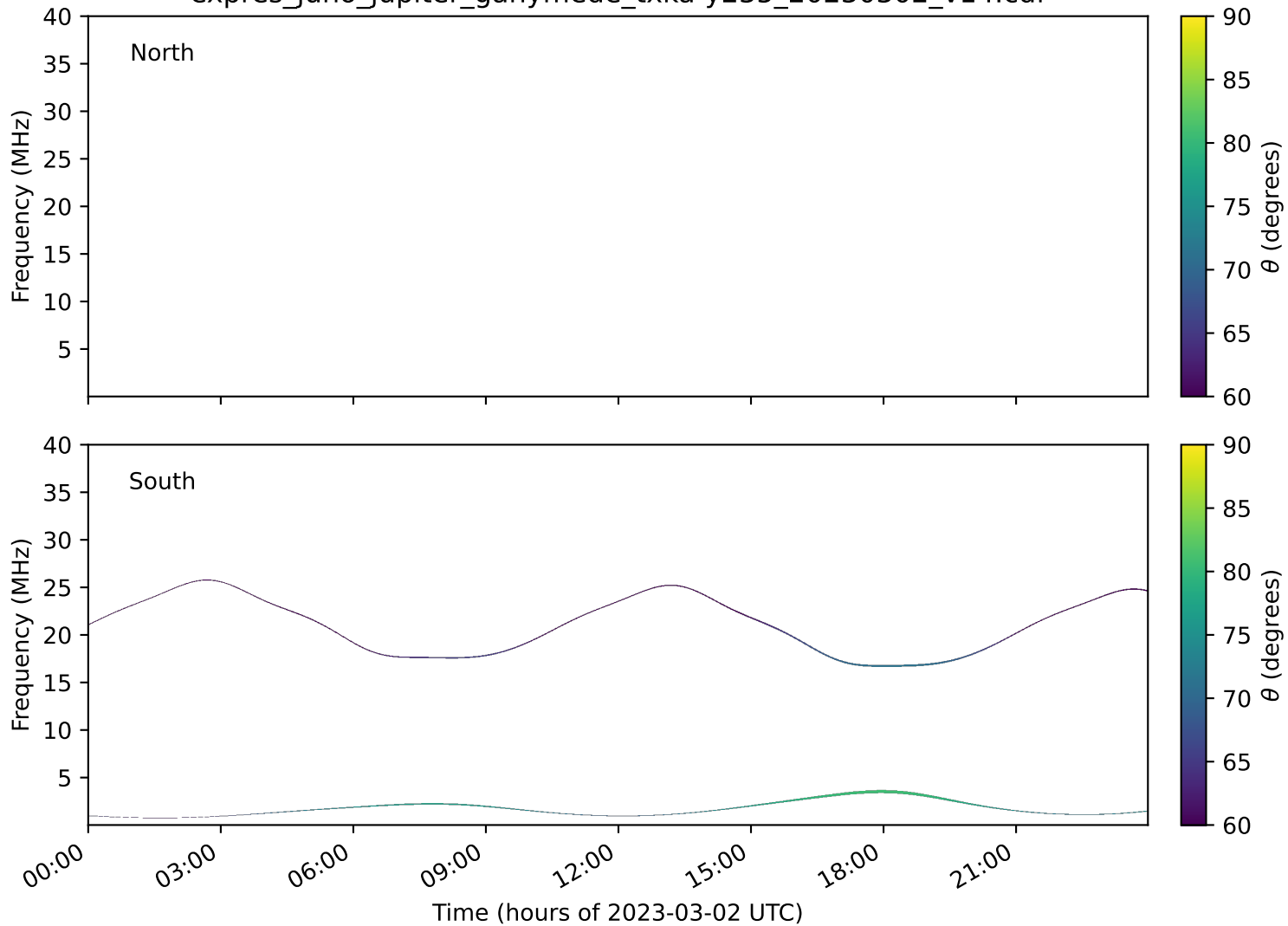
expres_juno_jupiter_ganymede_txka-y235_20230302_v14.cdf
