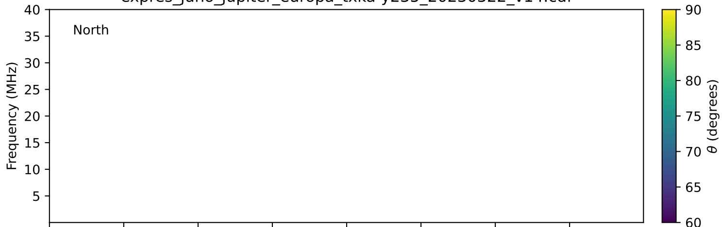
expres_juno_jupiter_europa_txka-y235_20230322_v14.cdf
