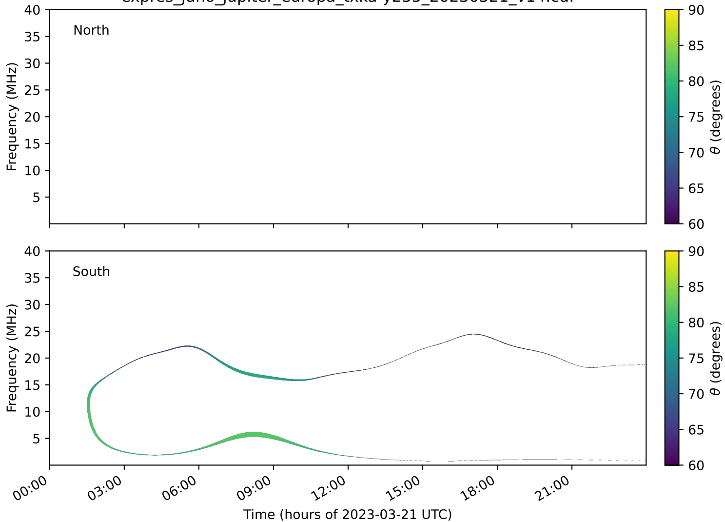
expres_juno_jupiter_europa_txka-y235_20230321_v14.cdf
