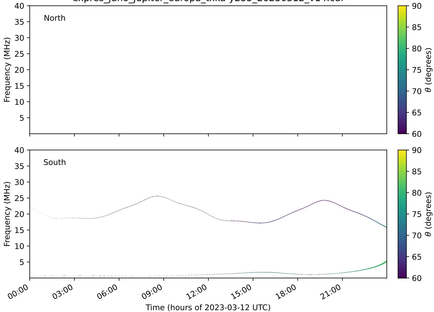
expres_juno_jupiter_europa_txka-y235_20230312_v14.cdf
