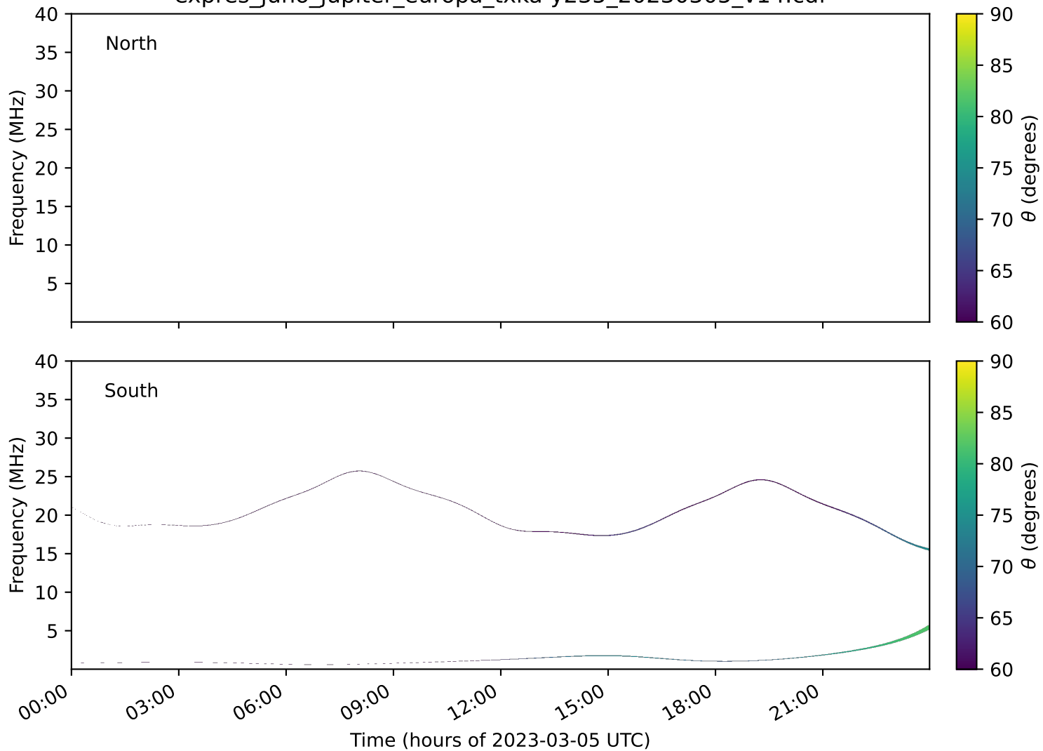
expres_juno_jupiter_europa_txka-y235_20230305_v14.cdf
