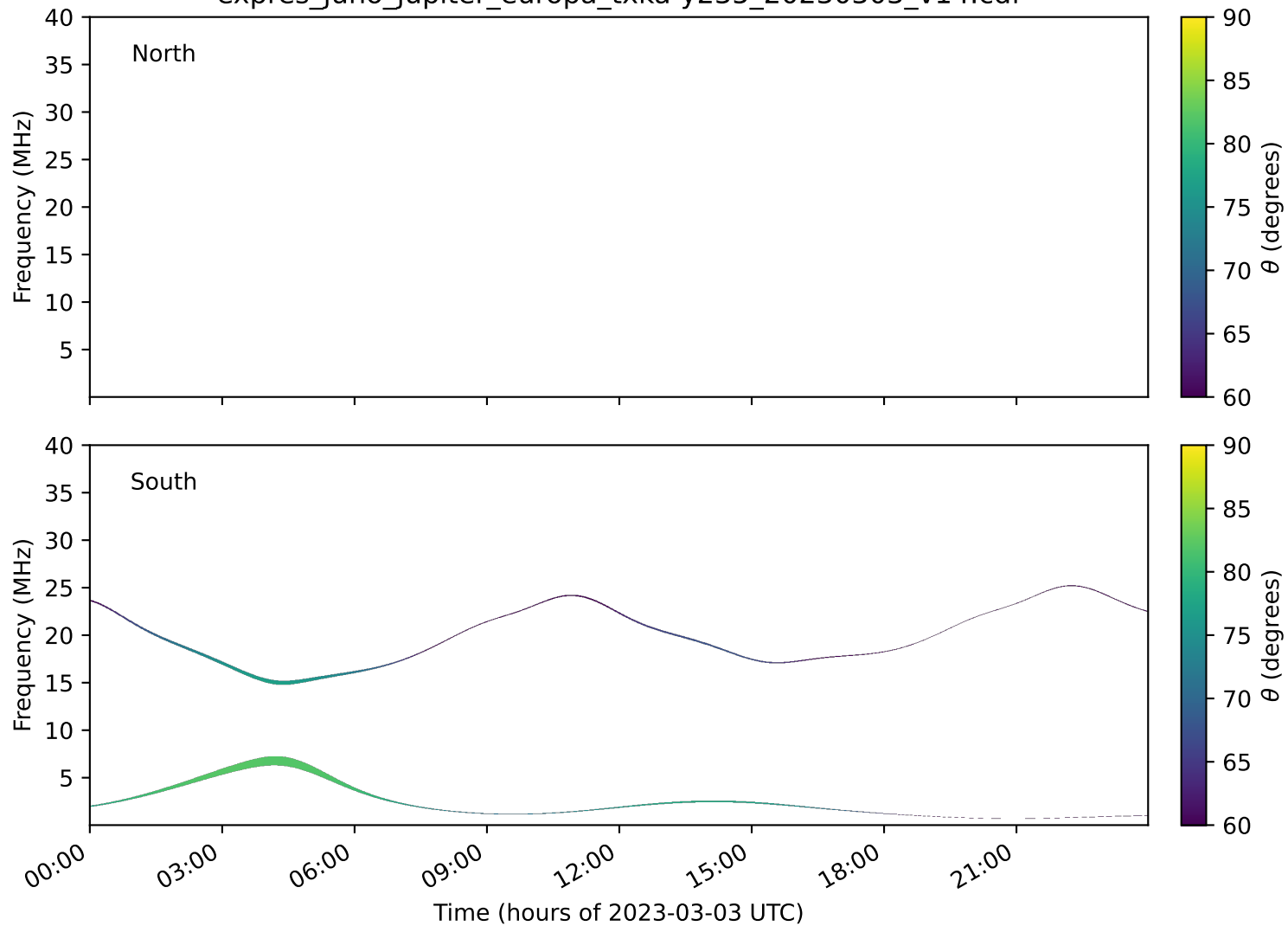
expres_juno_jupiter_europa_txka-y235_20230303_v14.cdf
