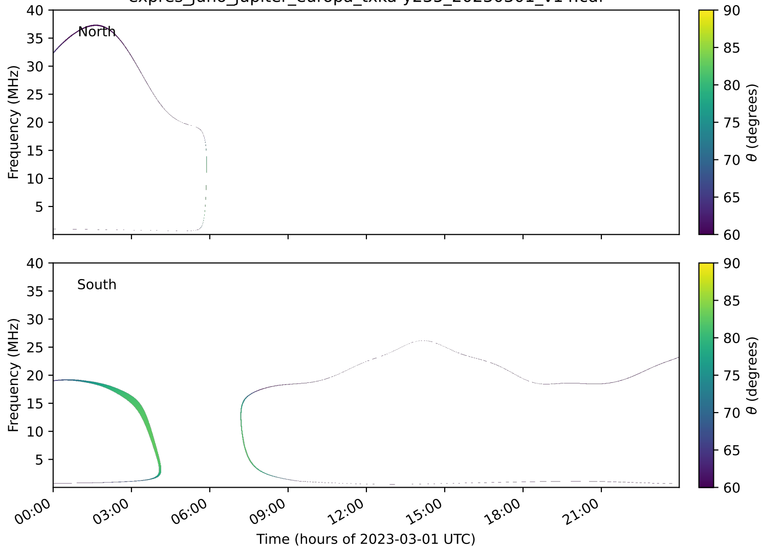
expres_juno_jupiter_europa_txka-y235_20230301_v14.cdf
