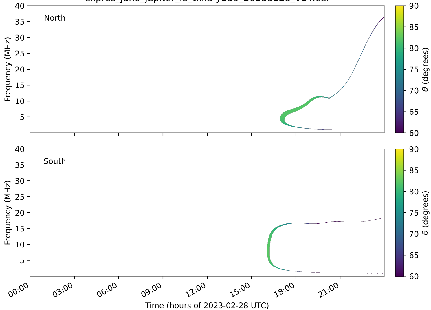
expres_juno_jupiter_io_txka-y235_20230228_v14.cdf
