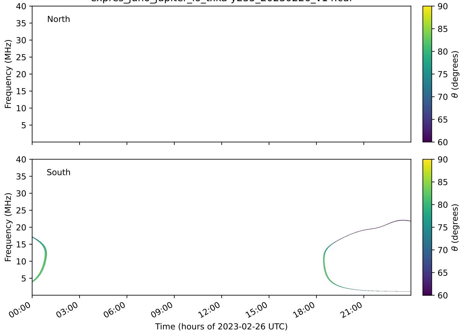
expres_juno_jupiter_io_txka-y235_20230226_v14.cdf
