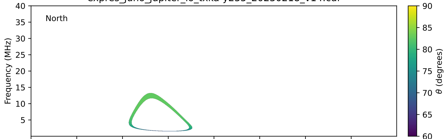
expres_juno_jupiter_io_txka-y235_20230218_v14.cdf
