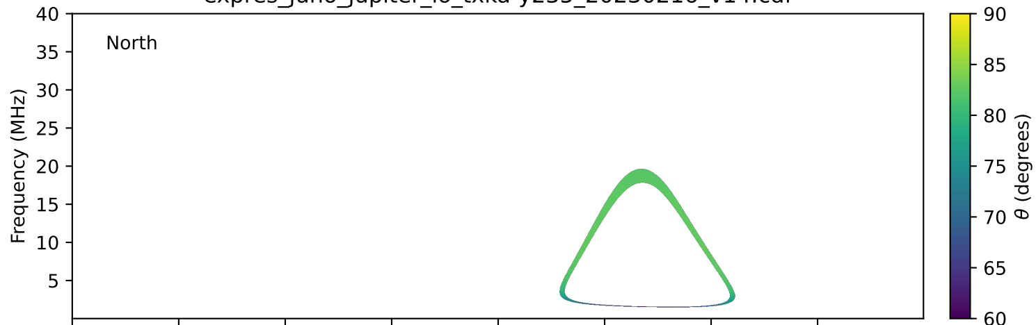
expres_juno_jupiter_io_txka-y235_20230216_v14.cdf
