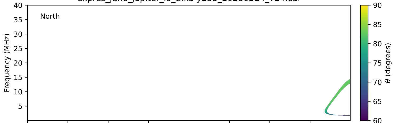
expres_juno_jupiter_io_txka-y235_20230214_v14.cdf
