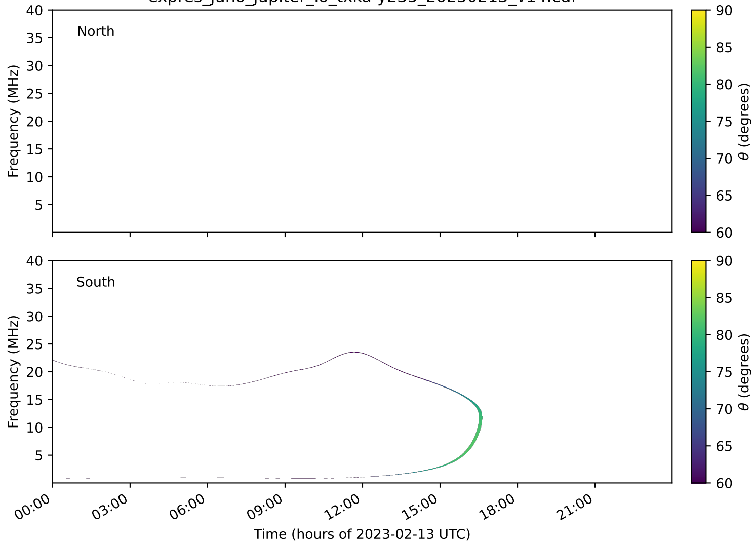
expres_juno_jupiter_io_txka-y235_20230213_v14.cdf
