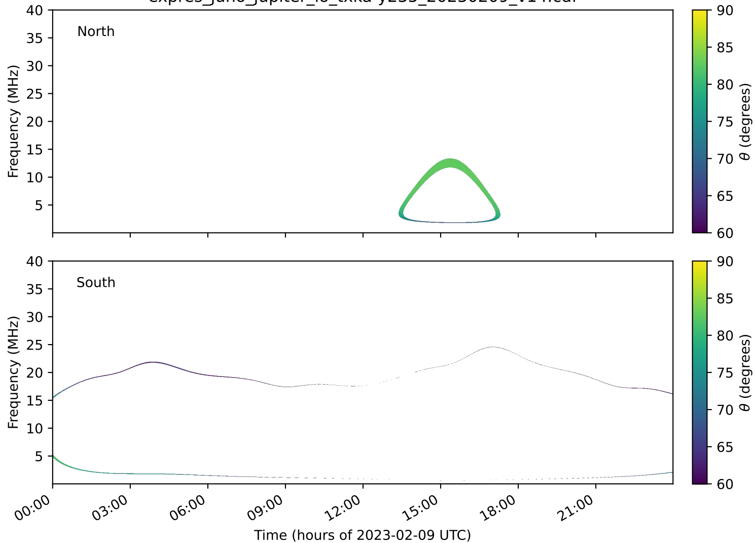
expres_juno_jupiter_io_txka-y235_20230209_v14.cdf
