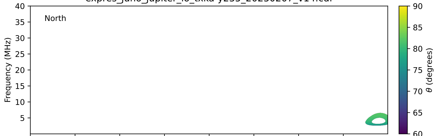
expres_juno_jupiter_io_txka-y235_20230207_v14.cdf
