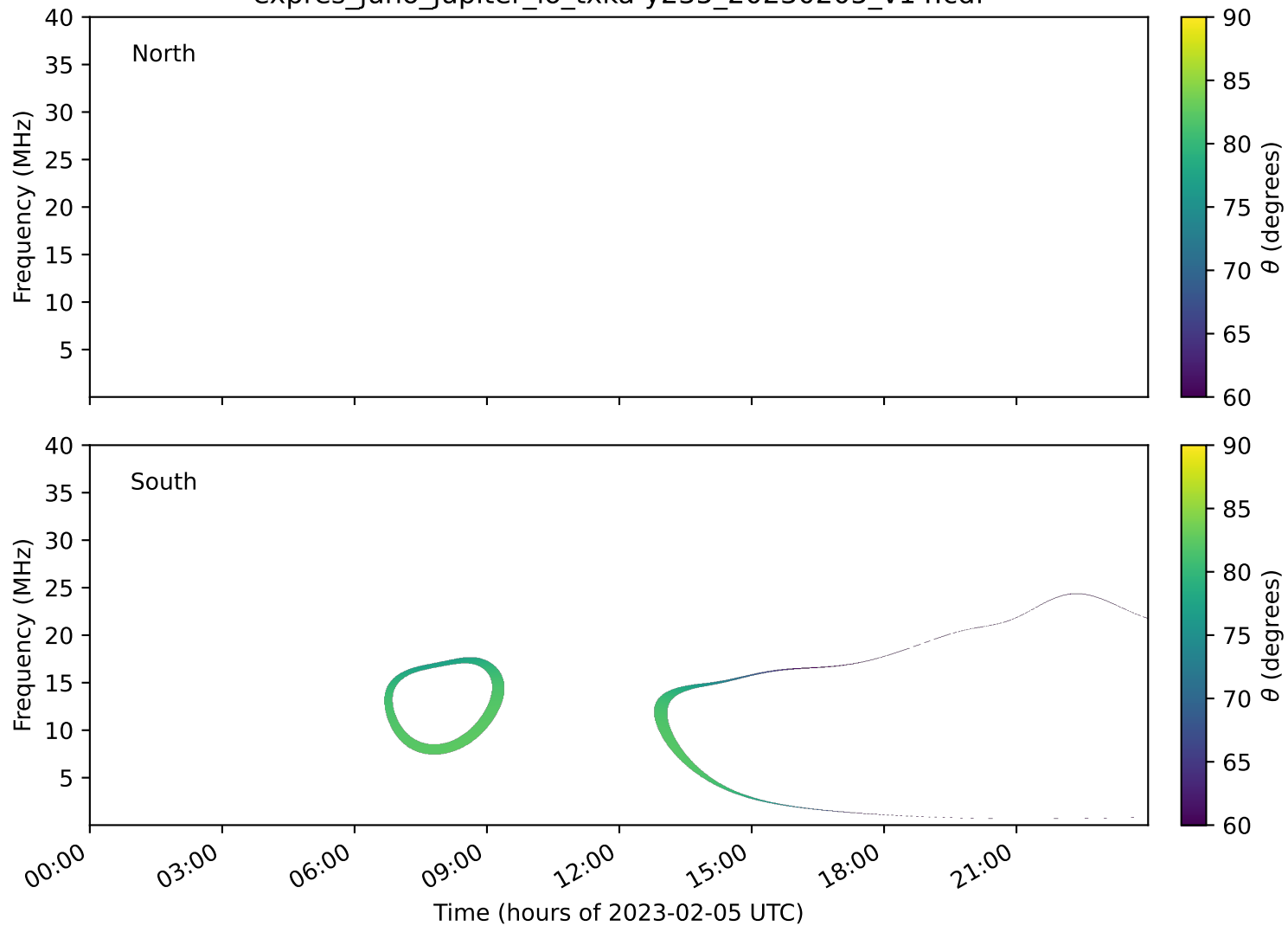
expres_juno_jupiter_io_txka-y235_20230205_v14.cdf
