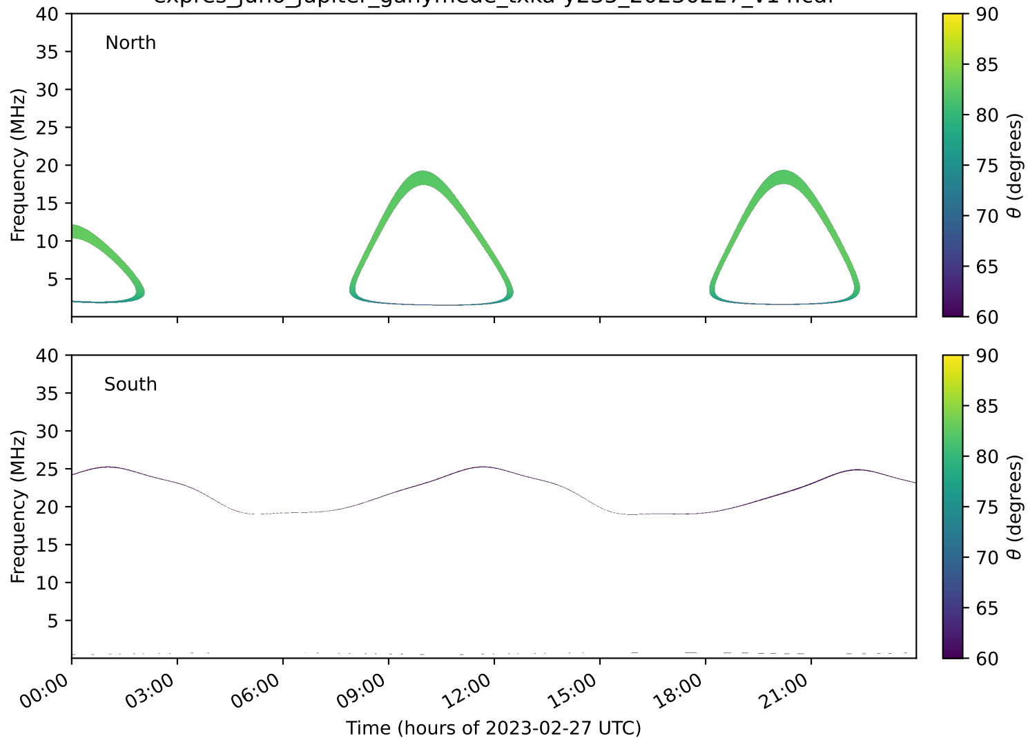
expres_juno_jupiter_ganymede_txka-y235_20230227_v14.cdf
