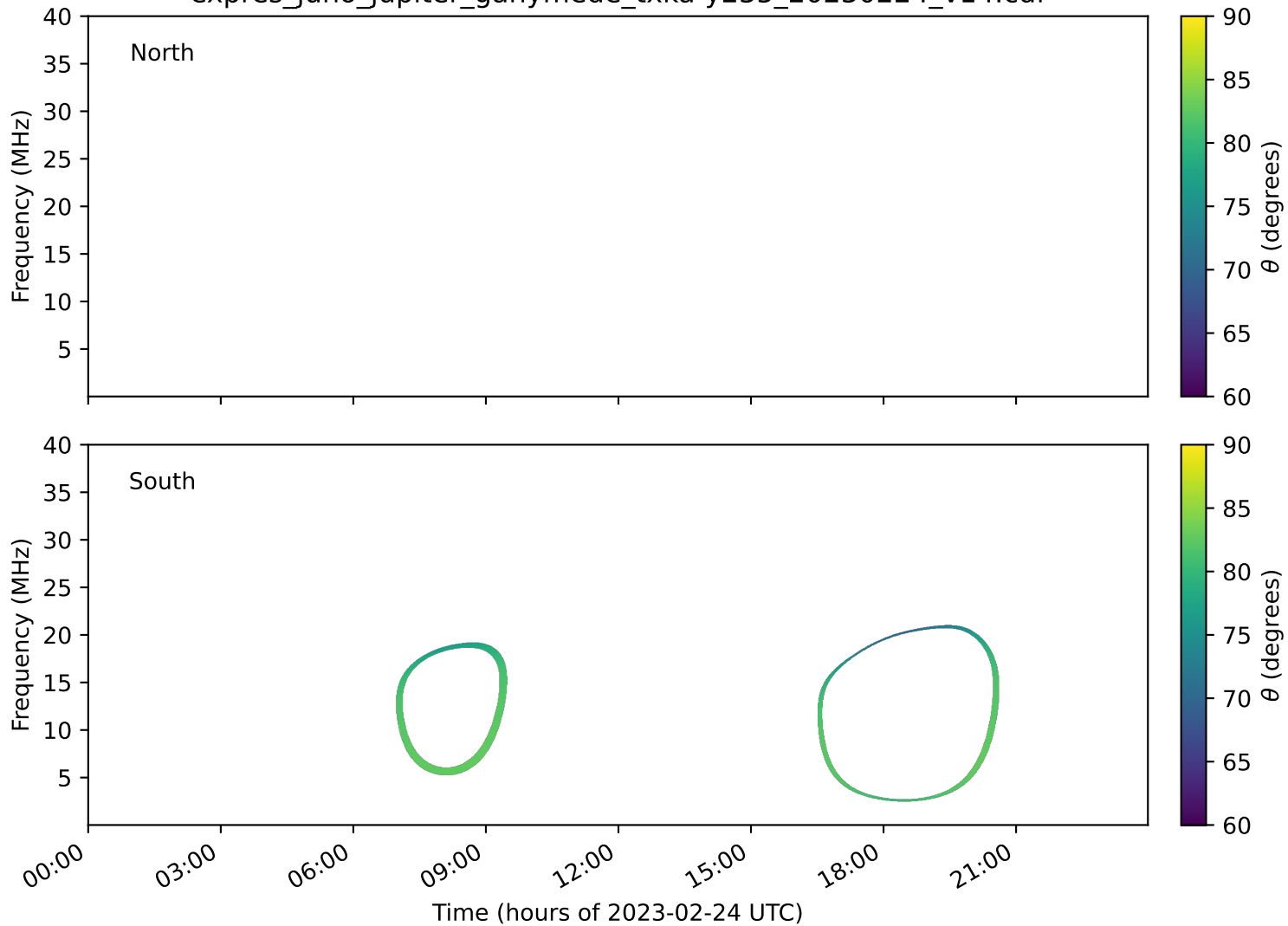
expres_juno_jupiter_ganymede_txka-y235_20230224_v14.cdf
