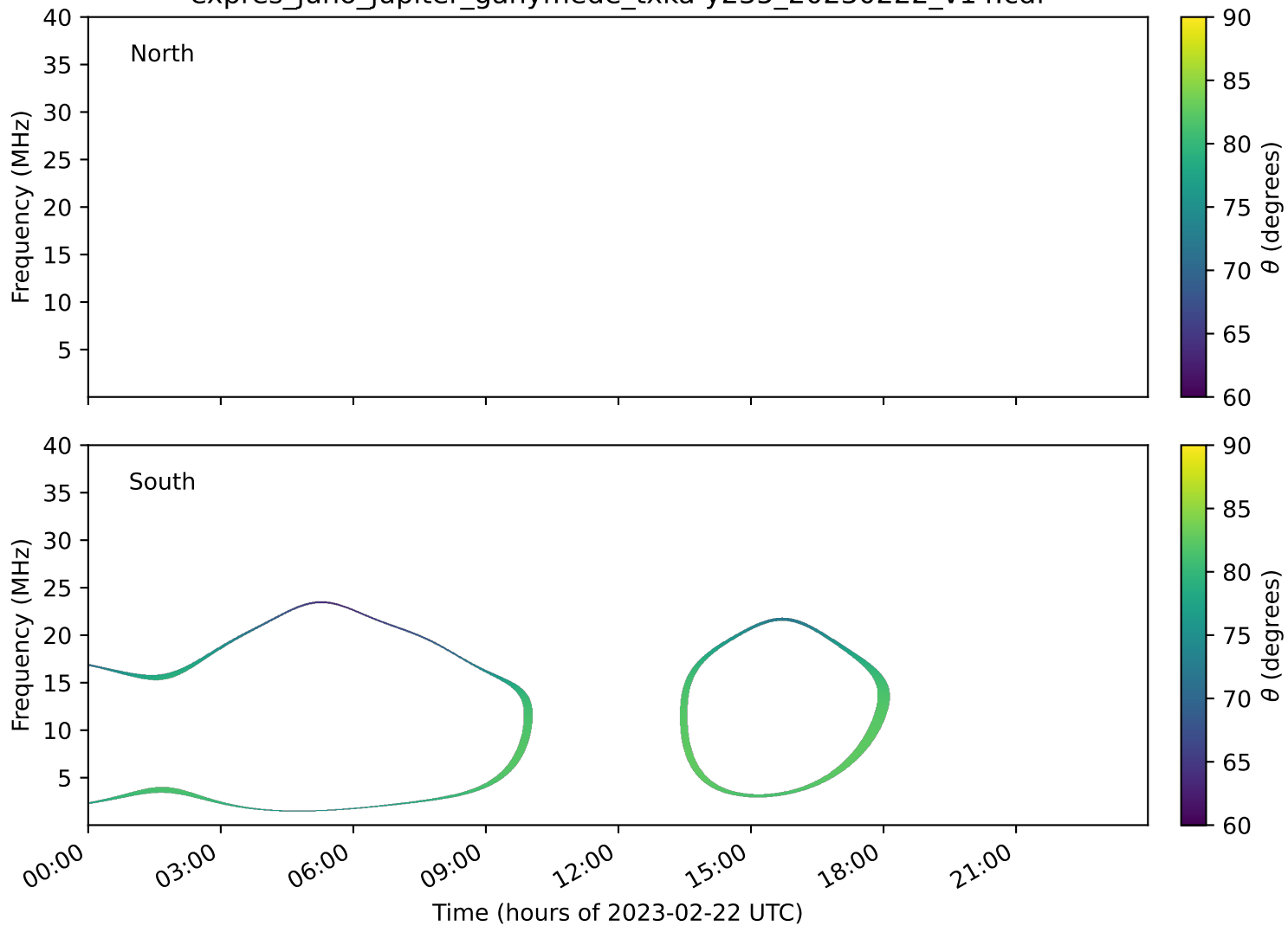
expres_juno_jupiter_ganymede_txka-y235_20230222_v14.cdf
