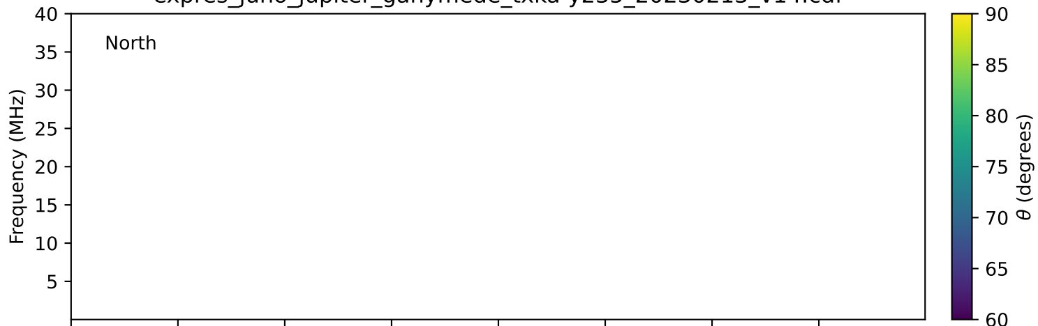
expres_juno_jupiter_ganymede_txka-y235_20230213_v14.cdf
