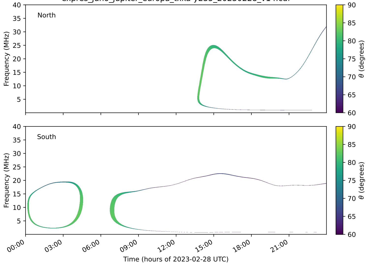
expres_juno_jupiter_europa_txka-y235_20230228_v14.cdf
