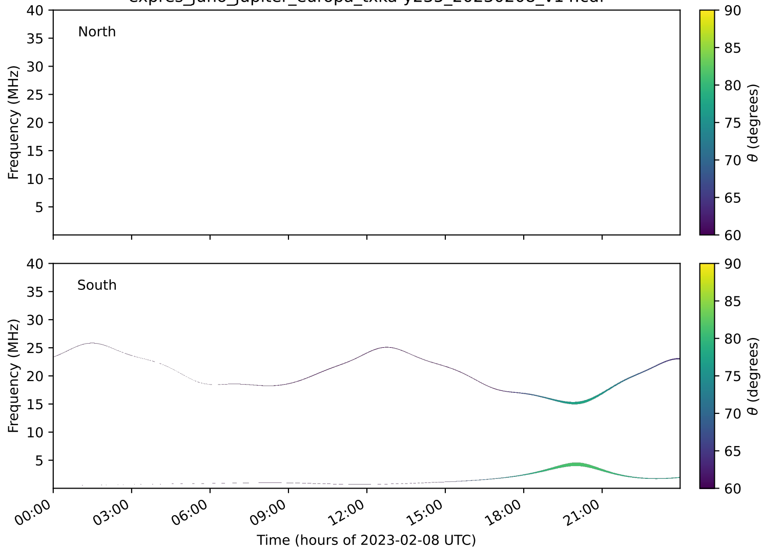
expres_juno_jupiter_europa_txka-y235_20230208_v14.cdf
