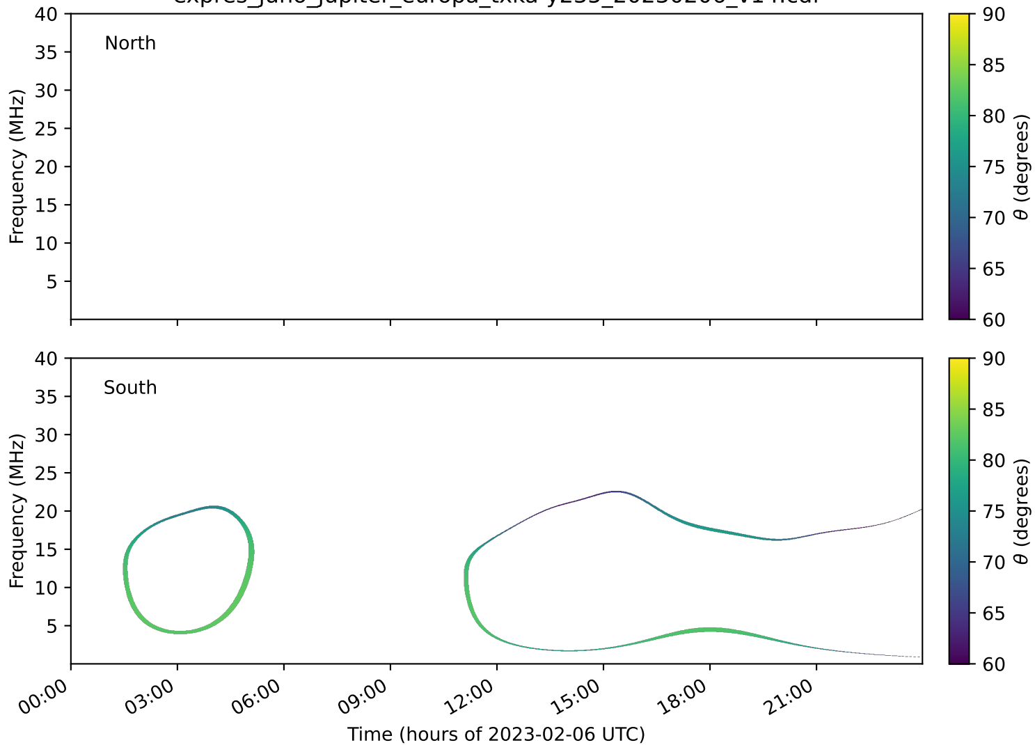
expres_juno_jupiter_europa_txka-y235_20230206_v14.cdf
