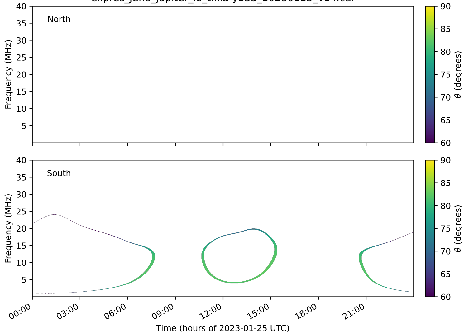
expres_juno_jupiter_io_txka-y235_20230125_v14.cdf
