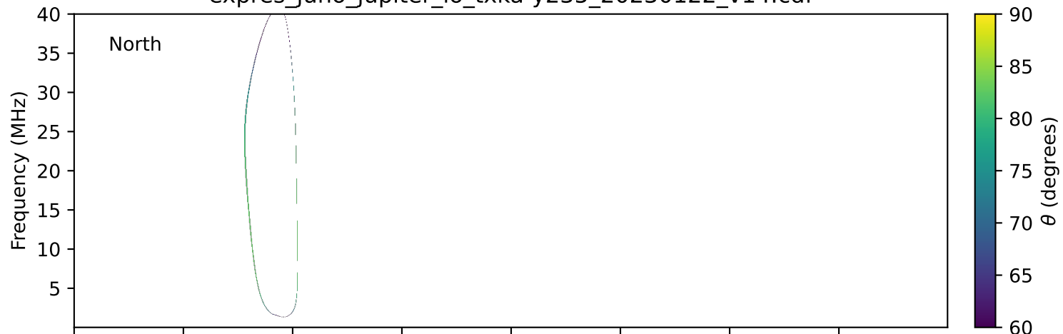
expres_juno_jupiter_io_txka-y235_20230122_v14.cdf
