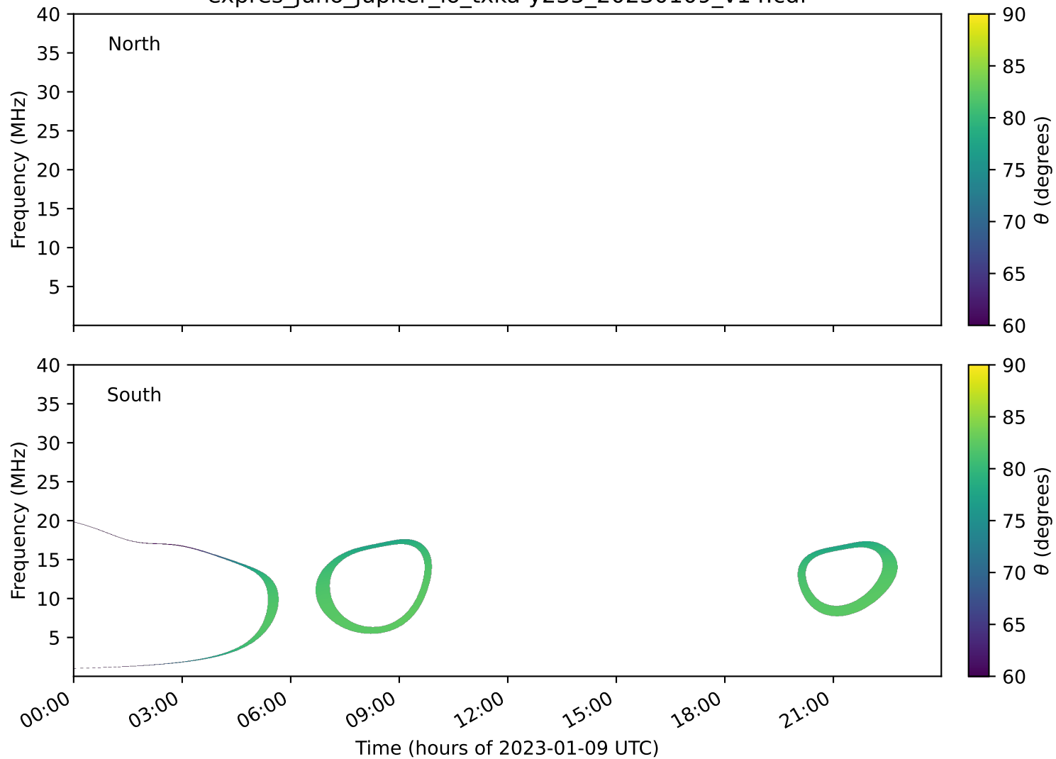
expres_juno_jupiter_io_txka-y235_20230109_v14.cdf
