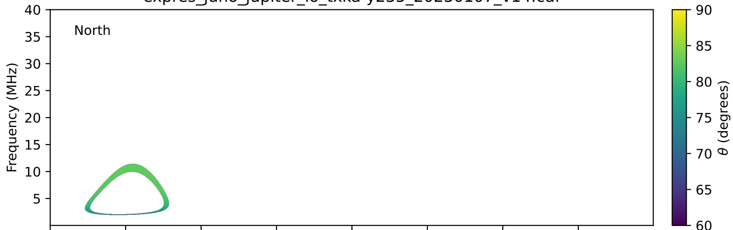
expres_juno_jupiter_io_txka-y235_20230107_v14.cdf
